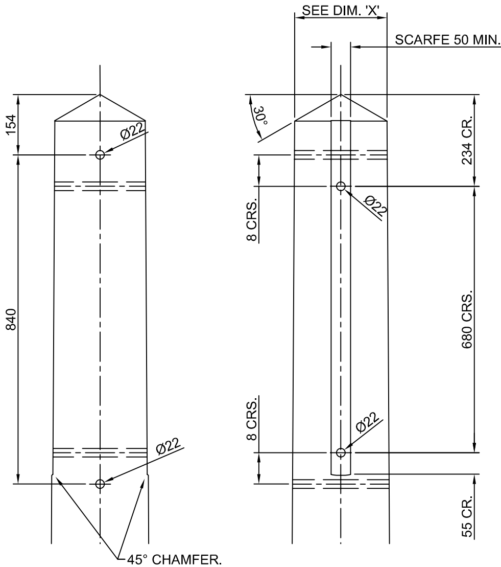
ENLARGED VIEWS OF POLE APEX SCALE 1:10
